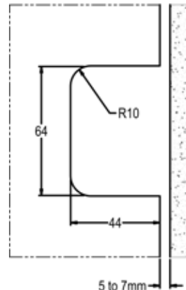
Glass Preparation
