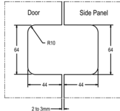
Glass Preparation
