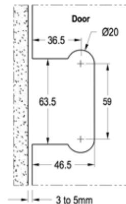
Glass Preparation
