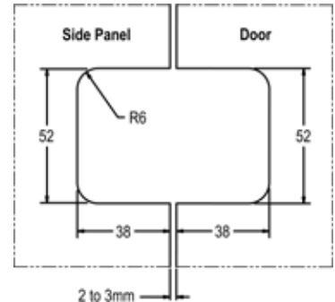
Glass Preparation
