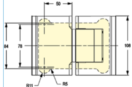
Glass Preparation
