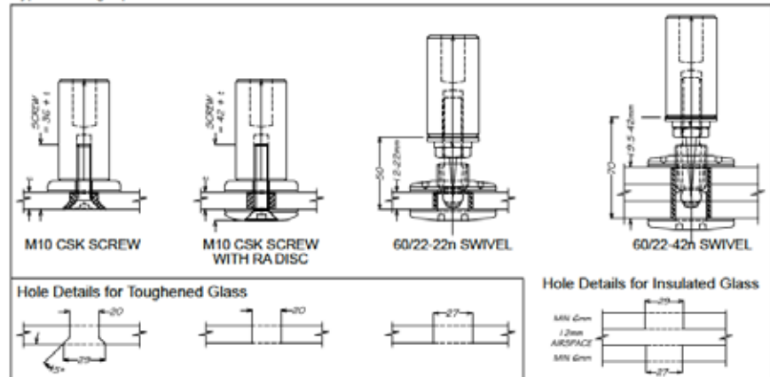
Glass Preparation
