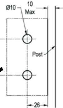
Glass Preparation
