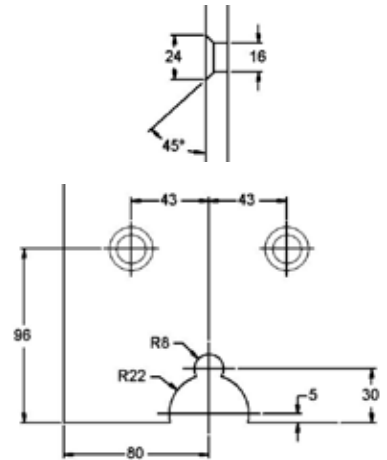
Glass Preparation
