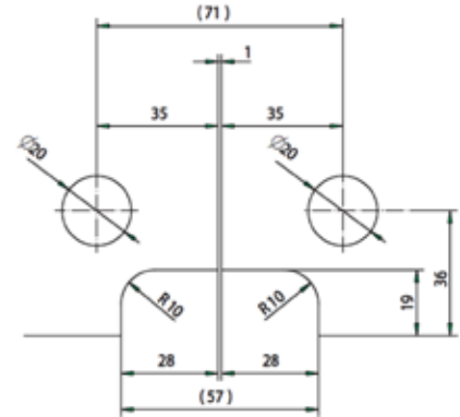
Glass Preparation
