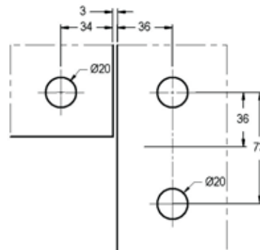
Glass Preparation
