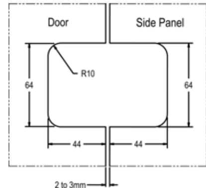
Glass Preparation
