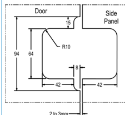
Glass Preparation
