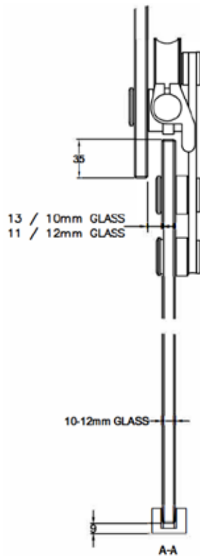
Dimensions &amp; Glass Preparation
