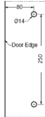
Glass Preparation
