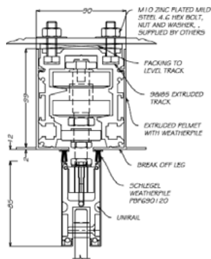
2 TOP RAIL SECTION SCALE: NTS
