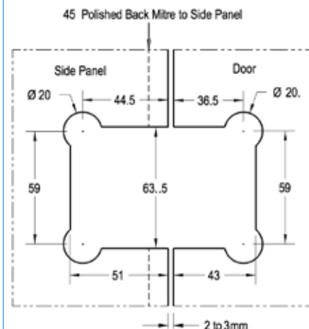
Glass Preparation
