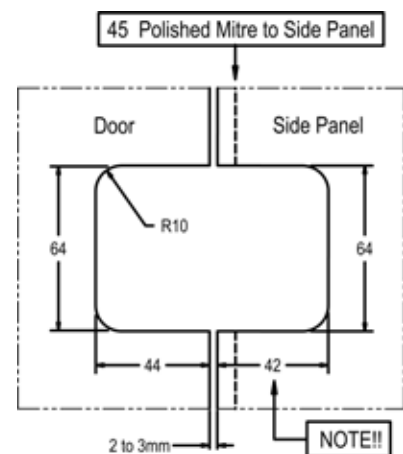
Glass Preparation
