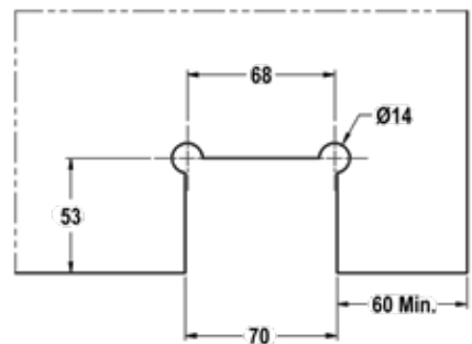
Glass Preparation
