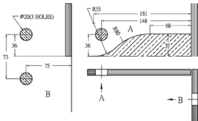
Glass Preparation (Left shown, right opposite setout)
