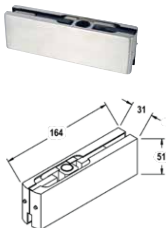
Product Image & Dimensions
