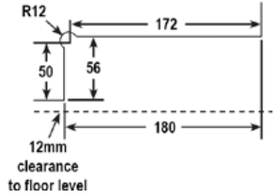
Glass Preparation
