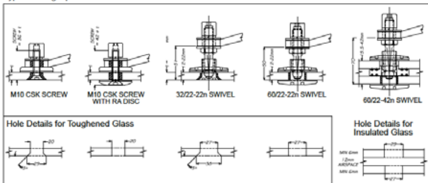
Glass Preparation
