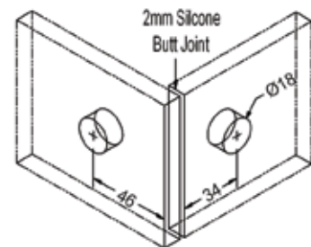
Glass Preparation
