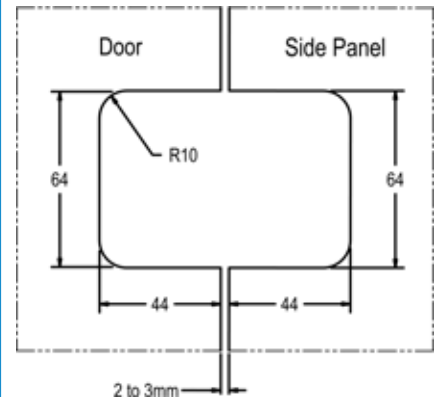
Glass Preparation
