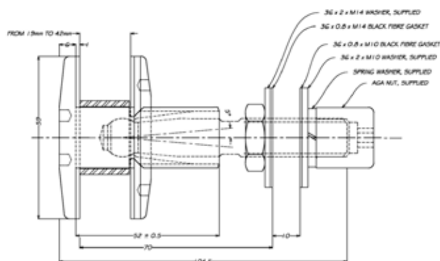
Product Image
