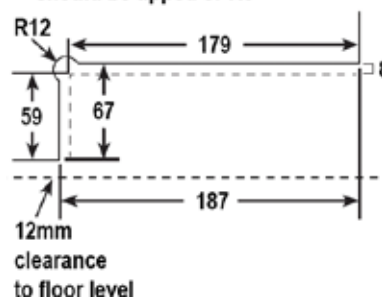
Glass Preparation
