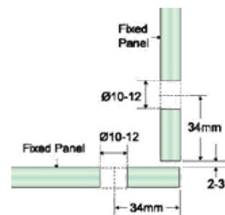
Glass Preparation
