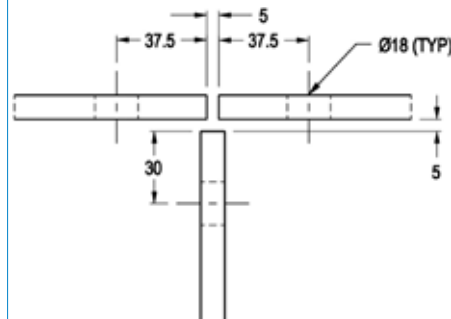
Glass Preparation
