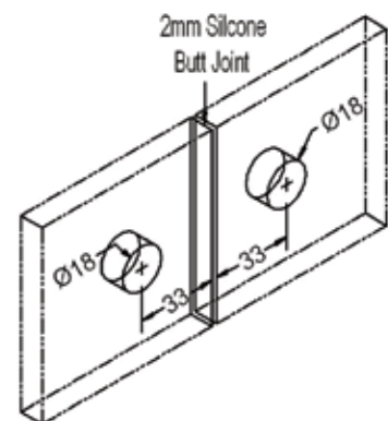
Glass Preparation
