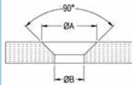
Glass Preparation
