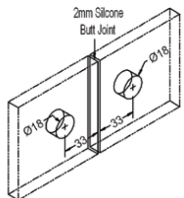
Glass Preparation
