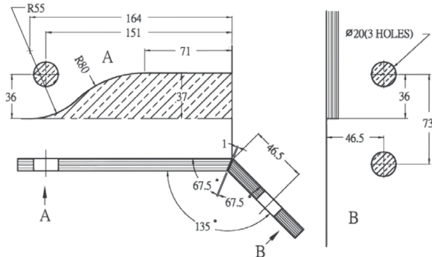
Glass Preparation (Left shown, right opposite setout)
