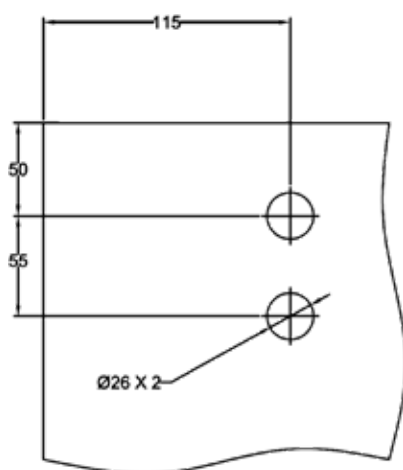
Glass Preparation - Carriage
