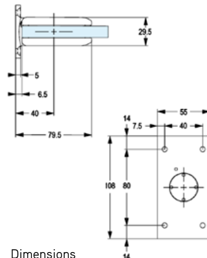
Glass Preparation
