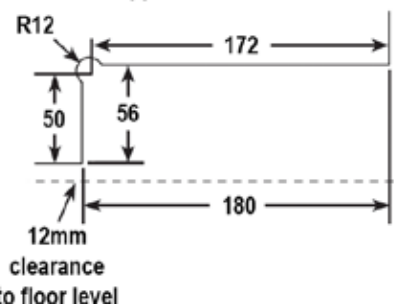
Glass Preparation
