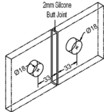
Glass Preparation
