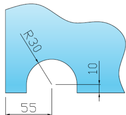
Glass Preparation
