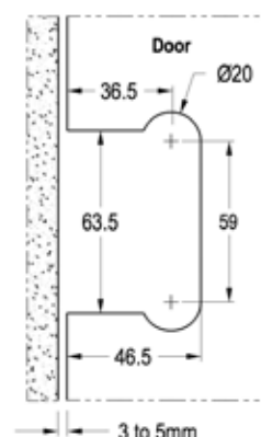
Glass Preparation
