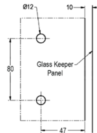
Glass Preparation
