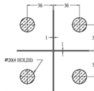
Glass Preparation
