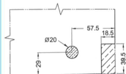
Glass Preparation
