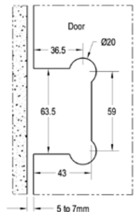
Glass Preparation
