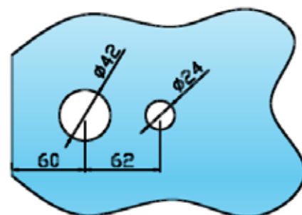
Glass Preparation
