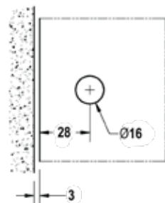
Glass Preparation
