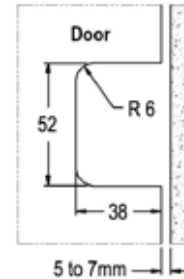
Glass Preparation
