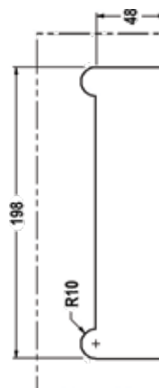
Glass Preparation
