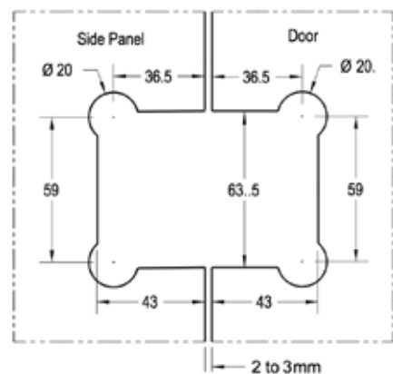
Glass Preparation
