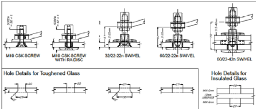
Glass Preparation
