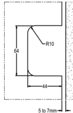
Glass Preparation
