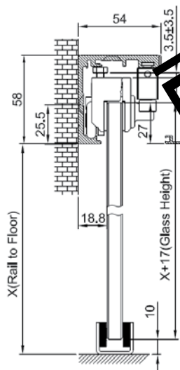
Wall Installation Dimensions & Glass Preparation
