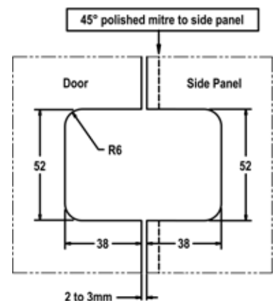
Glass Preparation
