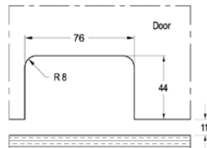
Glass Preparation
