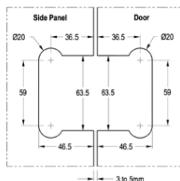
Glass Preparation
