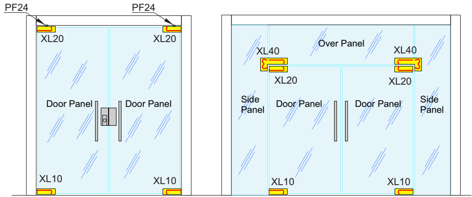
At Floor - Floor springs Dorma BTS80
